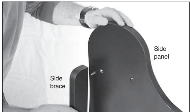
Figure 7. Attach a side brace to the outside of each side panel using three base assembly wood screws and the 4mm hex key.
