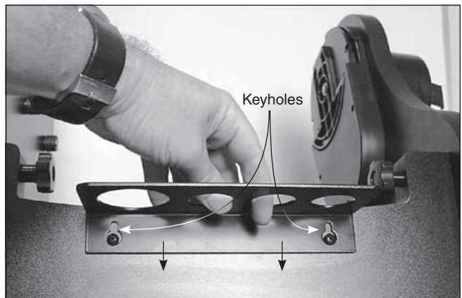
Figure 11. Place the large opening of the “keyhole” slots in the eyepiece rack over the mounting screw heads, then push the rack downward. To do this, leave the screw heads about 1/8” out from the panel. After the rack is installed, you can tighten the screws to secure it in place.
