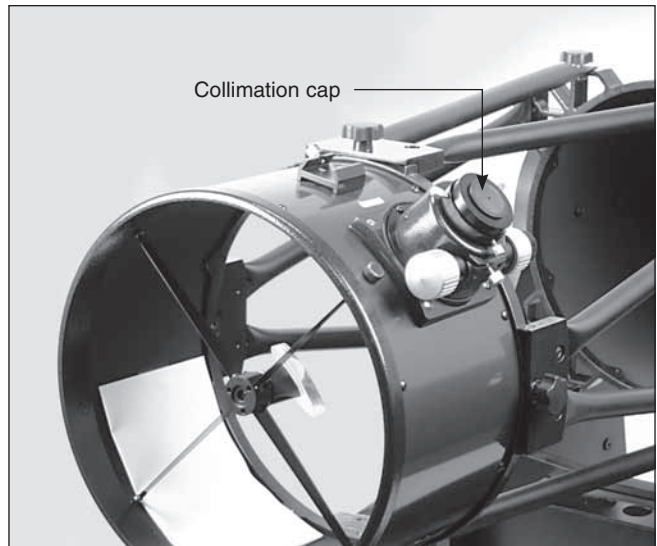
Figure 29. The SkyQuest optical tube properly set up for collimation.
