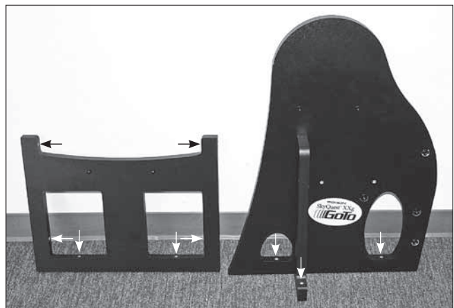
Figure 8. Locations for connecting bolts in the front and side panels (one side panel not shown). Connecting bolts should be inserted in the predrilled holes in the direction indicated by the arrows.
