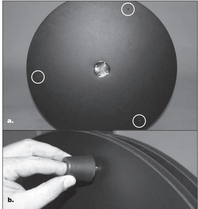
Figure 6. a) Starter holes for feet on bottom baseplate. b) Attaching the base feet.
