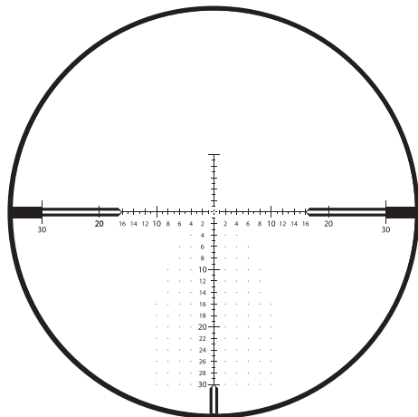
ZF-MOAI = ZEISS First Focal Plane – Minute of Angle, illuminated
